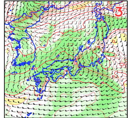
<24>2918UTC T850,TTd850,W850
