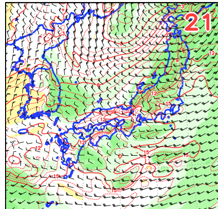
<42>3012UTC T850,TTd850,W850
