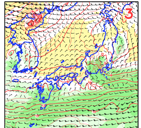
<72>0118UTC T850,TTd850,W850
