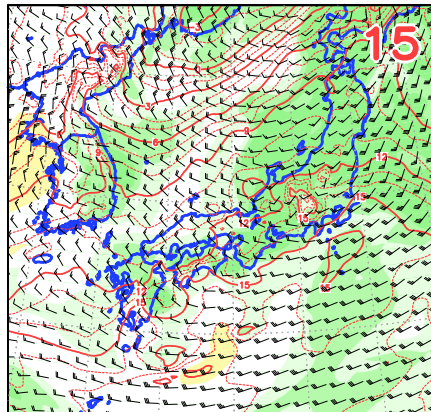
<36>3006UTC T850,TTd850,W850
