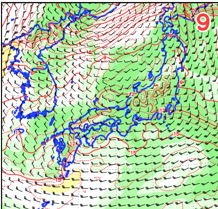
<30>3000UTC T850,TTd850,W850
