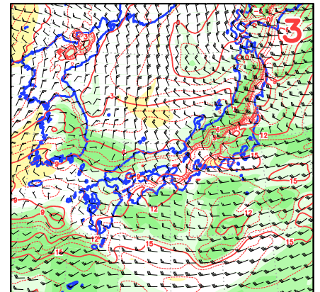
<48>3018UTC T850,TTd850,W850
