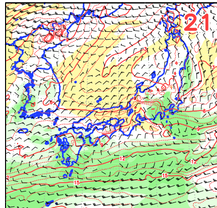
<66>0112UTC T850,TTd850,W850
