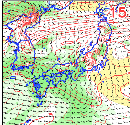
<12>2906UTC T850,TTd850,W850
