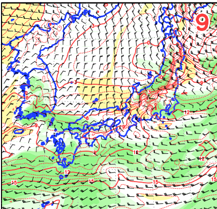
<54>0100UTC T850,TTd850,W850
