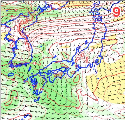
<6>2900UTC T850,TTd850,W850
