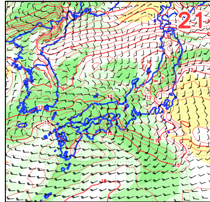
<18>2912UTC T850,TTd850,W850
