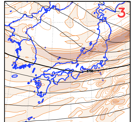
<72>0118UTC Z500 Vor500
