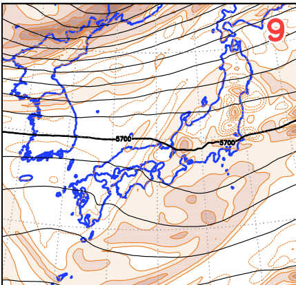
<30>3000UTC Z500 Vor500
