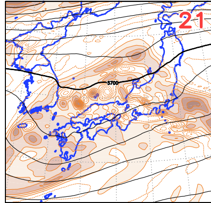
<18>2912UTC Z500 Vor500
