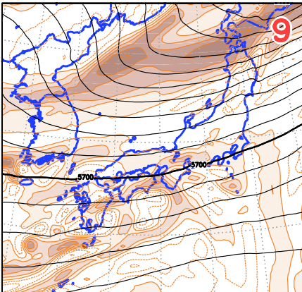
<54>0100UTC Z500 Vor500
