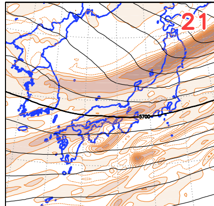
<66>0112UTC Z500 Vor500
