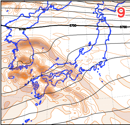
<6>2900UTC Z500 Vor500
