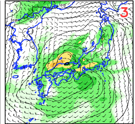
<24>2918UTC Psea Wind R6
