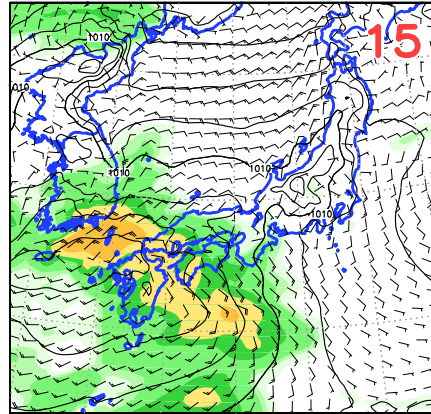
<12>2906UTC Psea Wind R6
