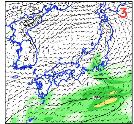
<72>0118UTC Psea Wind R6
