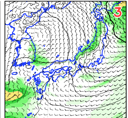
<48>3018UTC Psea Wind R6
