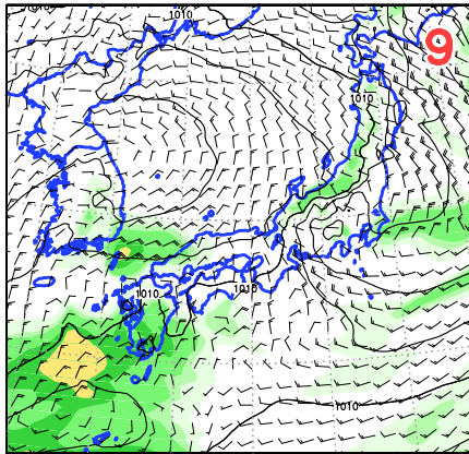
<54>0100UTC Psea Wind R6
