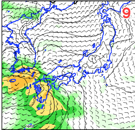
<6>2900UTC Psea Wind R6
