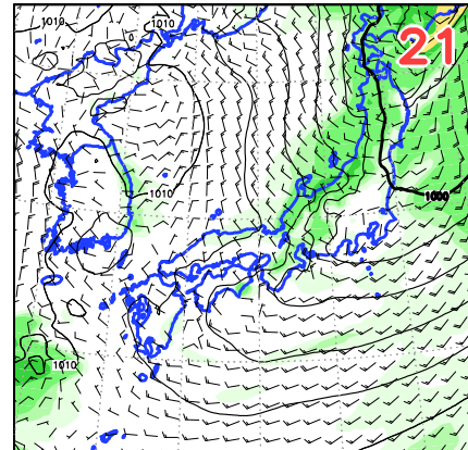
<42>3012UTC Psea Wind R6
