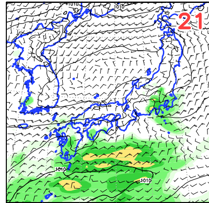
<66>0112UTC Psea Wind R6
