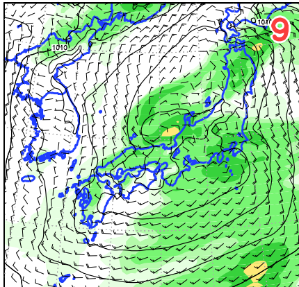
<30>3000UTC Psea Wind R6
